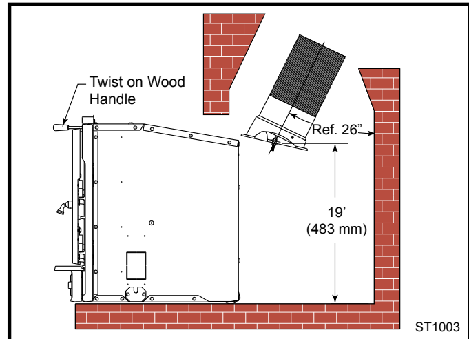
Fig. 7 Measured height from the finished hearth surface to the center bar of the flue collar.
