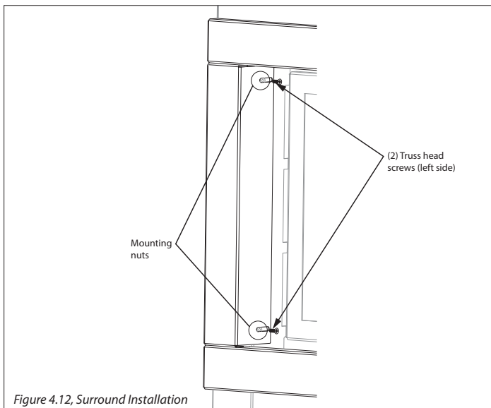
Figure 4.12, Surround Installation
