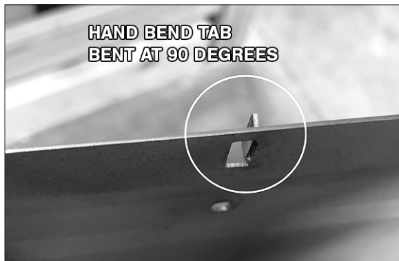
Figure 4.6, Hand Bend Tab
