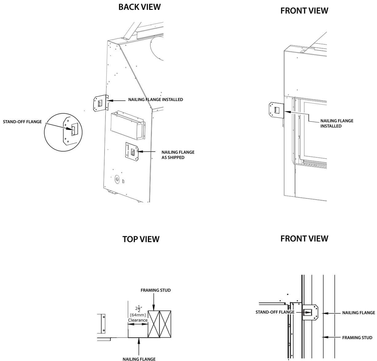
Figure 3.3, Nailing Flange Installation
