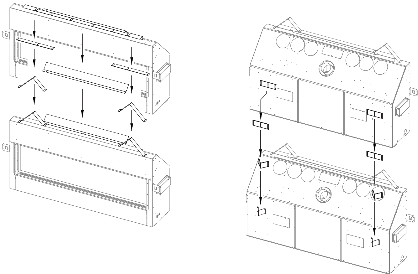
Figure 3.2, Stand-off Assembly and Installation
