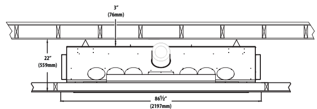
TYPICAL VERTICAL INSTALLATION
