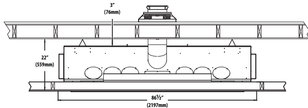
TYPICAL HORIZONTAL TERMINATION
