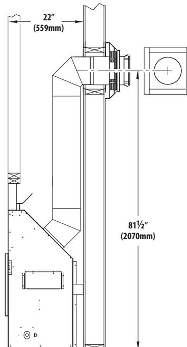
PROPANE RIGID PIPE MINIMUM HORIZONTAL TERMINATION
