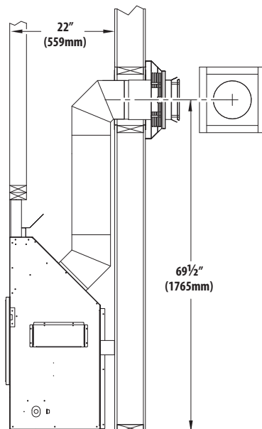
NATURAL GAS RIGID PIPE MINIMUM HORIZONTAL TERMINATION
