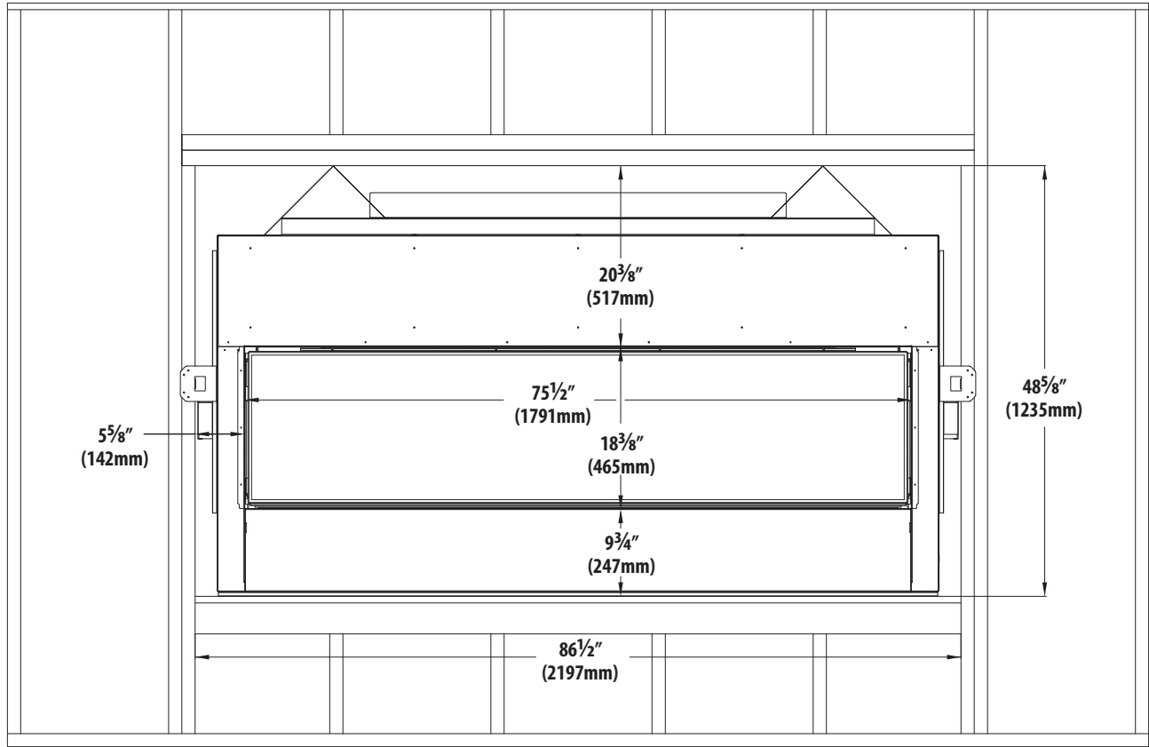
Figure 4.3, Finished Opening Clearances
